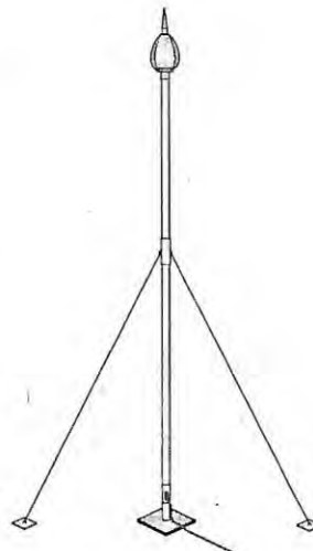
Figure 37. Guyed Mast
