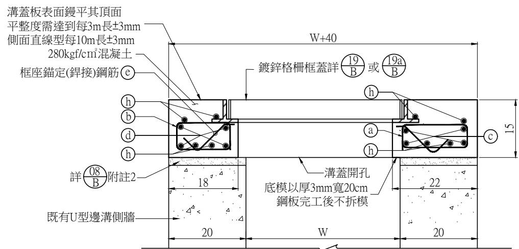
S 2型場鑄溝蓋板詳圖(板厚15cm) A1 (1:5) A3 (1:10) Unit:cm
