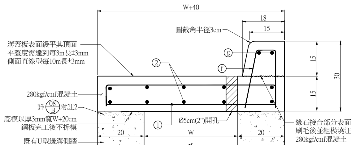
L 1型場鑄溝蓋板剖面圖(板厚15cm) A1 (1:5) A3 (1:10) Unit:cm
