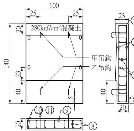
乙種預鑄溝蓋版詳圖 A1 (1:20) A3 (1:40) Unit:cm
