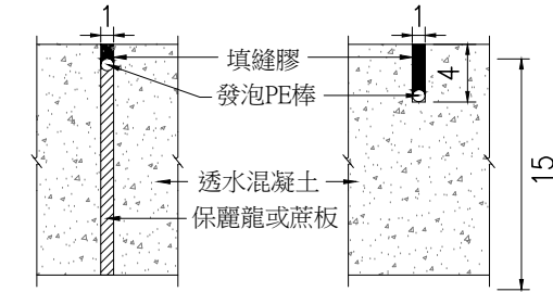
透水混凝土伸縮縫及縮縫詳圖 NTS Unit:cm
