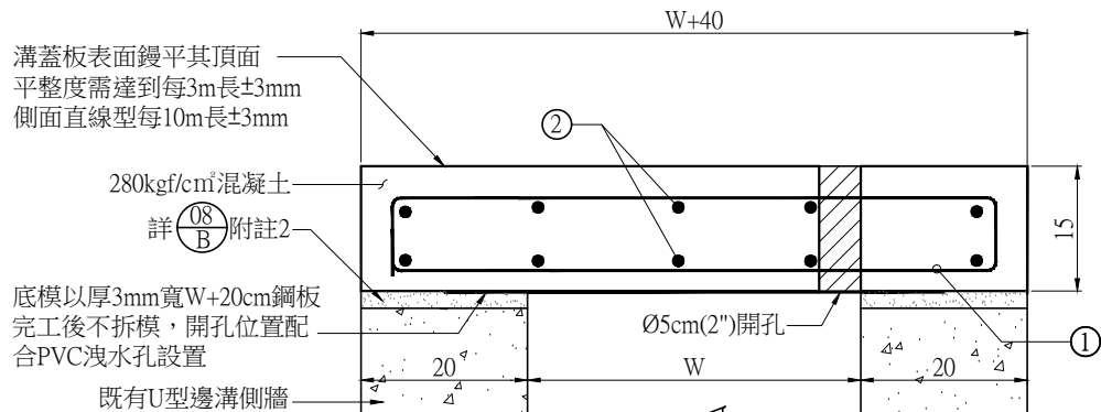
S 1型場鑄溝蓋板詳圖(板厚15cm) A1 (1:5) A3 (1:10) Unit:cm
