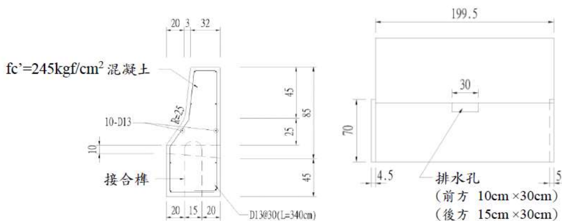
斷面及配筋
